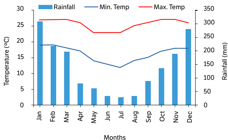
Figure 1. Average data of a 30-year series of maximum and minimum temperatures and accumulated monthly rainfall of the municipality of São Sebastião da Grama, SP, Brazil.
