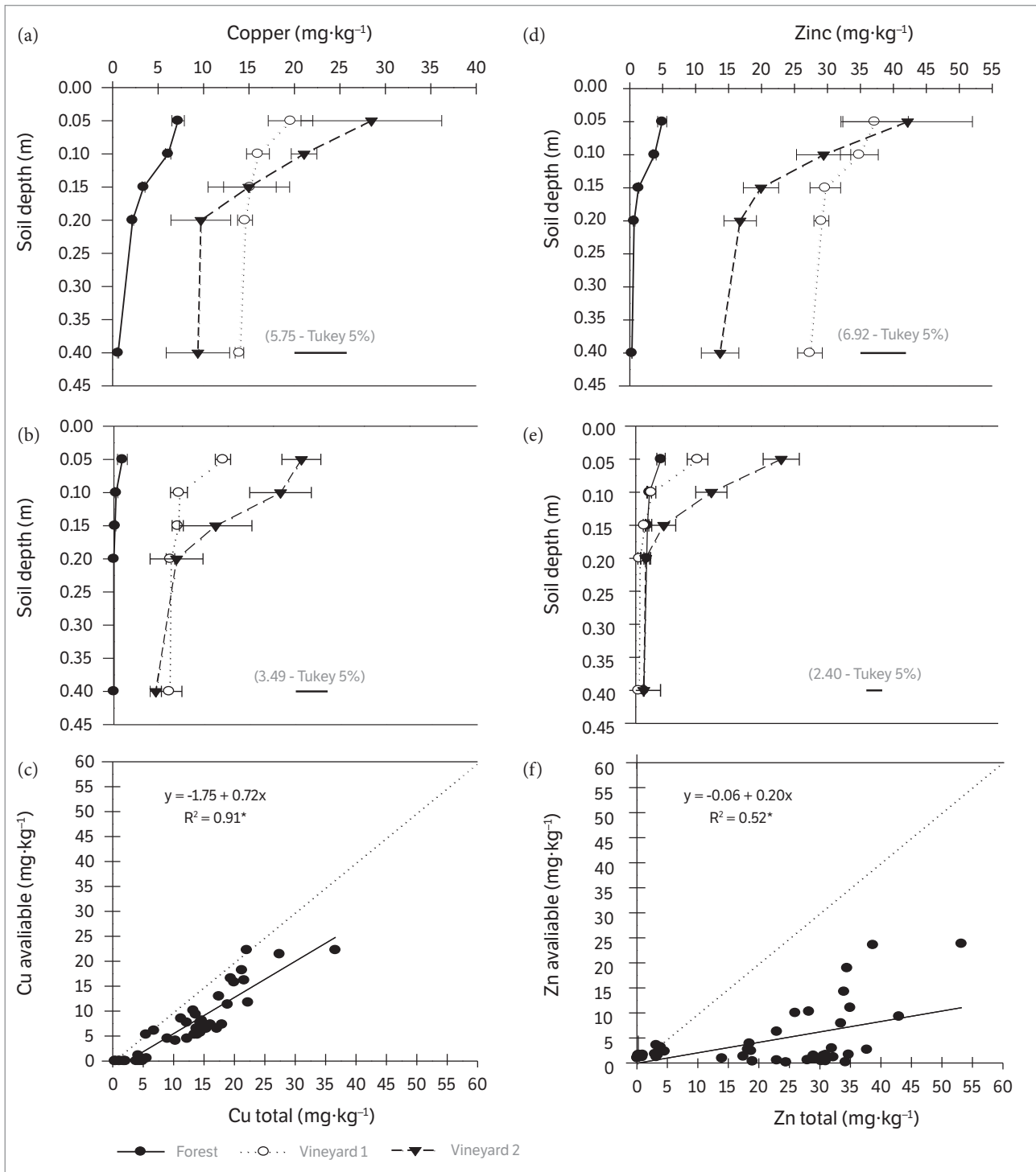
Figure 1. (a) Total copper content (CuEPA); (b) copper available to plants (CuEDTA); (c) correlation between CuEPA and CuEDTA at all depths (n=45); (d) total zinc (ZnEPA); (e) zinc available to plants (ZnEDTA) and (f) correlation between ZnEPA and ZnEDTA at all depths (n=72), in the forest, vineyard 1 (4 years) and vineyard 2 (15 years) soils; (*= means \pm standard deviation do not differ from each other according to Tukey's test p < 0.05 ). Bars represent standart deviation of the mean. Dashed line represents reference line.
