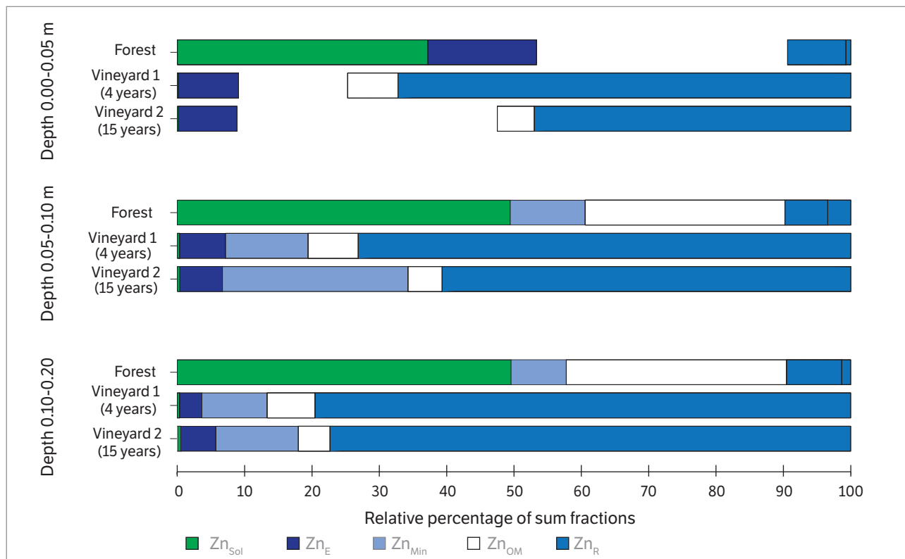
Figure 3. Percent average distribution of Zn fractions ( Zn_E exchangeable; Zn_{Sol} soluble; Zn_{Min} bonded to oxides; Zn_{OM} bonded to organic matter and Zn_R residual Zn) in soil layers of the forest, vineyard 1 (4 years) and vineyard 2 (15 years).
