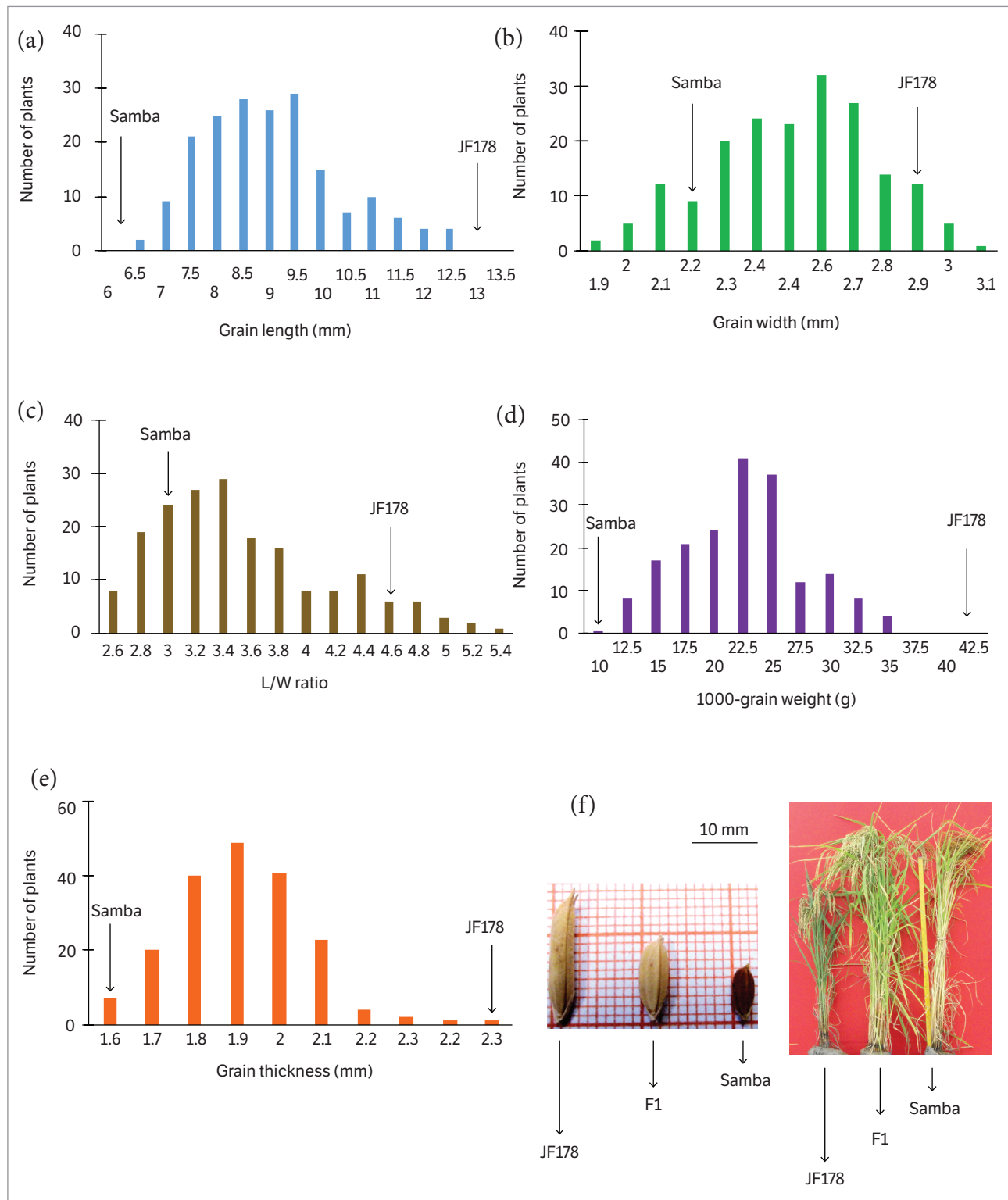
Figure 3. Characterization of grain traits in the JF178/Samba population. The long-grain mutant JF178 was crossed to the very short-grain cultivar Samba. The mean values of grain length, L/W ratio, grain thickness and 1000 kernel weight for F 1 plants were intermediate between those of the two parents, whereas grain width of F 1 was close to that of JF178. In the F 2 population of 186 plants, grain length fell between the two parents and exhibited a bimodal distribution trend (a). Grain width exhibited a certain degree of transgressive segregation and an approximate normal distribution (b). Both the L/W ratio and 1000 kernel weight displayed transgressive segregation and skewed distribution (c-d). Grain thickness did not show a transgressive segregation and exhibited an approximate normal distribution (e). Representative images of grains and plants of JF178, Samba and their F 1 are shown in (f-g).
